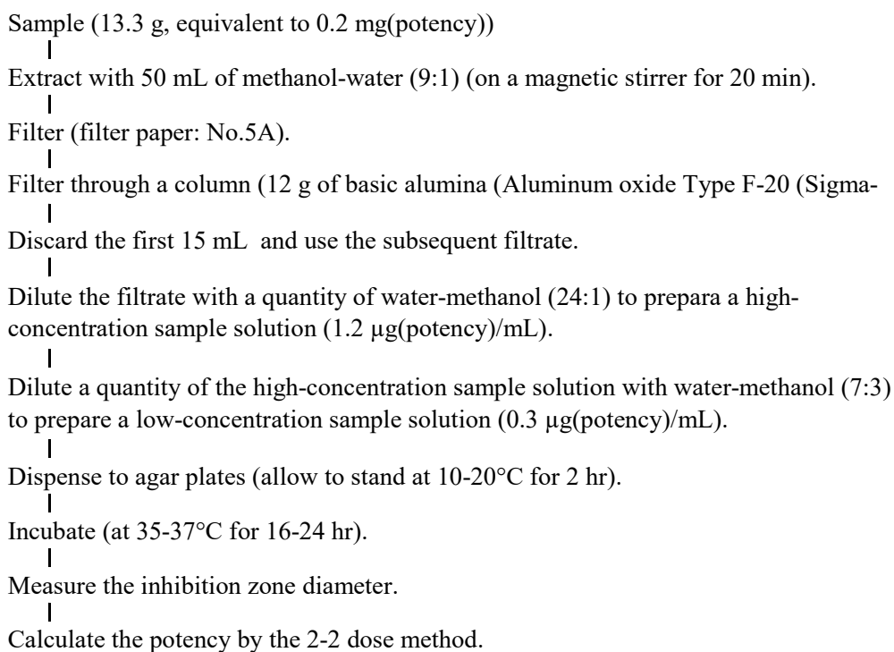
Figure 9.2.13-5 Quantitative test method for salinomycin sodium (cattle feed)
