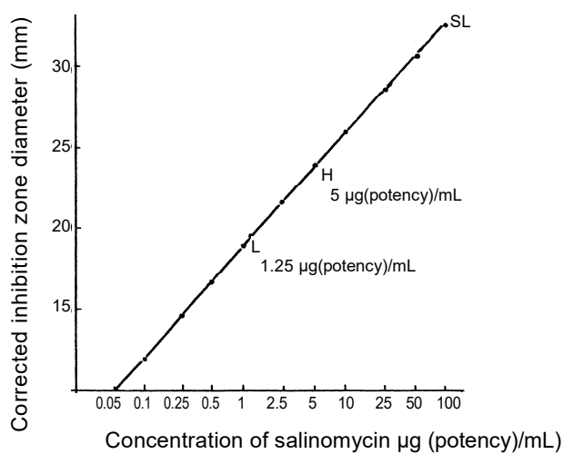
Figure 9.2.13-2 Standard response line for salinomycin (premix, example)
