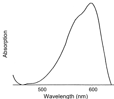
Figure 9.2.13-7 Absorption spectrum of chromogenic substrate for salinomycin (solvent: ethanol)
