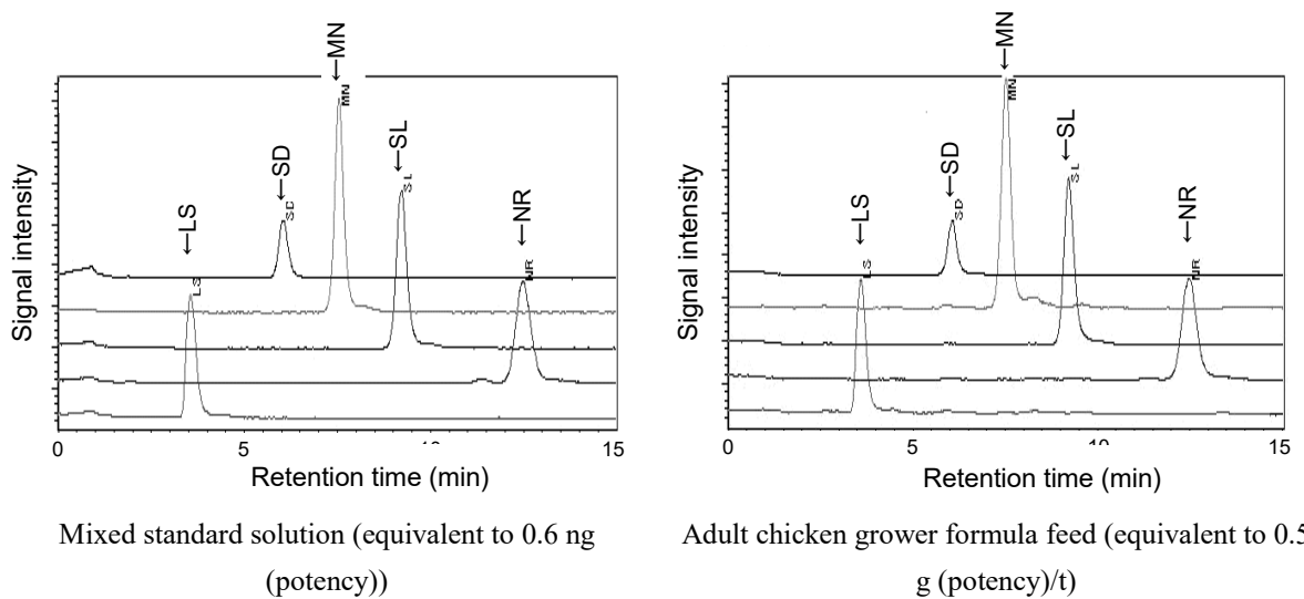
Figure 9.3.4-3 SIM chromatograms for the mixed standard solution and sample solution
