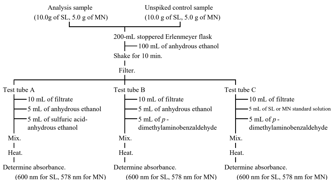
Figure 9.2.13-6 Rapid quantitative method for salinomycin and monensin (feed)
