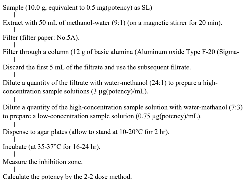
Figure 9.2.13-3 Quantification method for salinomycin sodium (chicken feed)
